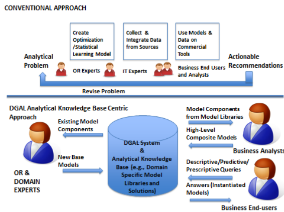
Figure 1: Conventional Approach vs. DGAL Approach
